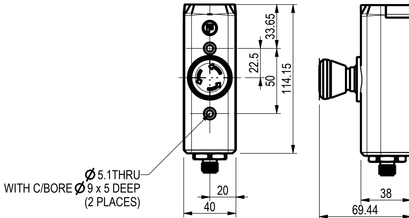
Dimensional Drawing - TEC, TED, TEW, TEV, TET, TEM, TEP, TEI, TES
