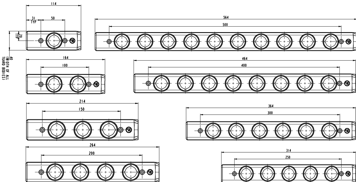
Figure 1: Dimensional Drawing - Bodies
